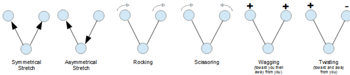
Illustration 1: Vibrational modes of molecules
