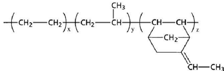
Illustration 2: Chemical structure of an EPDM molecule
